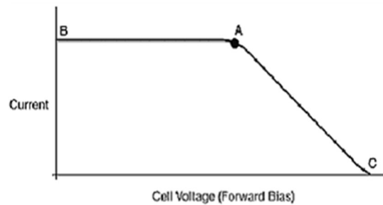
Fig 1.4 Illustration of Maximum power point
