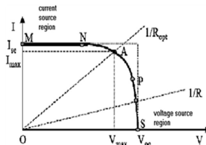
Fig.1.1 Solar cell Characteristics
