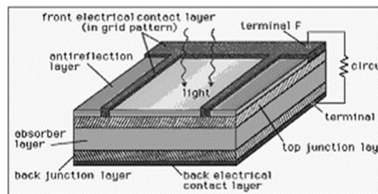
Fig.1 Solar cell
