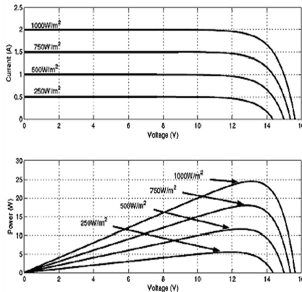
Fig 1.2 I-V and P-V characteristics of a solar cell for various irradiance
