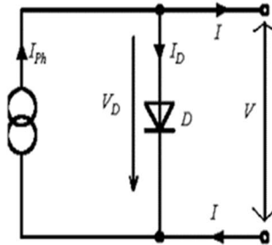
Fig 1.5. Equivalent circuit of solar cell
